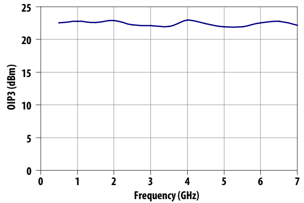
Figure 6. Output IP3 [1,2]
